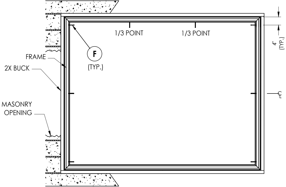
FRAME ANCHORING (2X BUCK)
