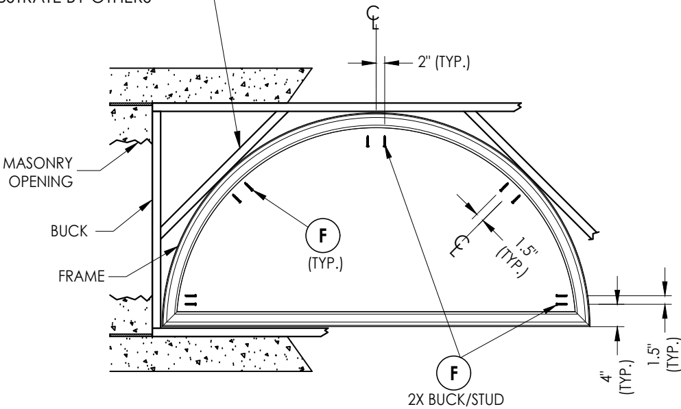
FRAME ANCHORING 72" X 40" MAX. 2X BUCK/2X STUD
